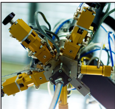
Mixing Head
